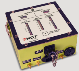
Airlock Control Module (ACM) – H018160-YY
